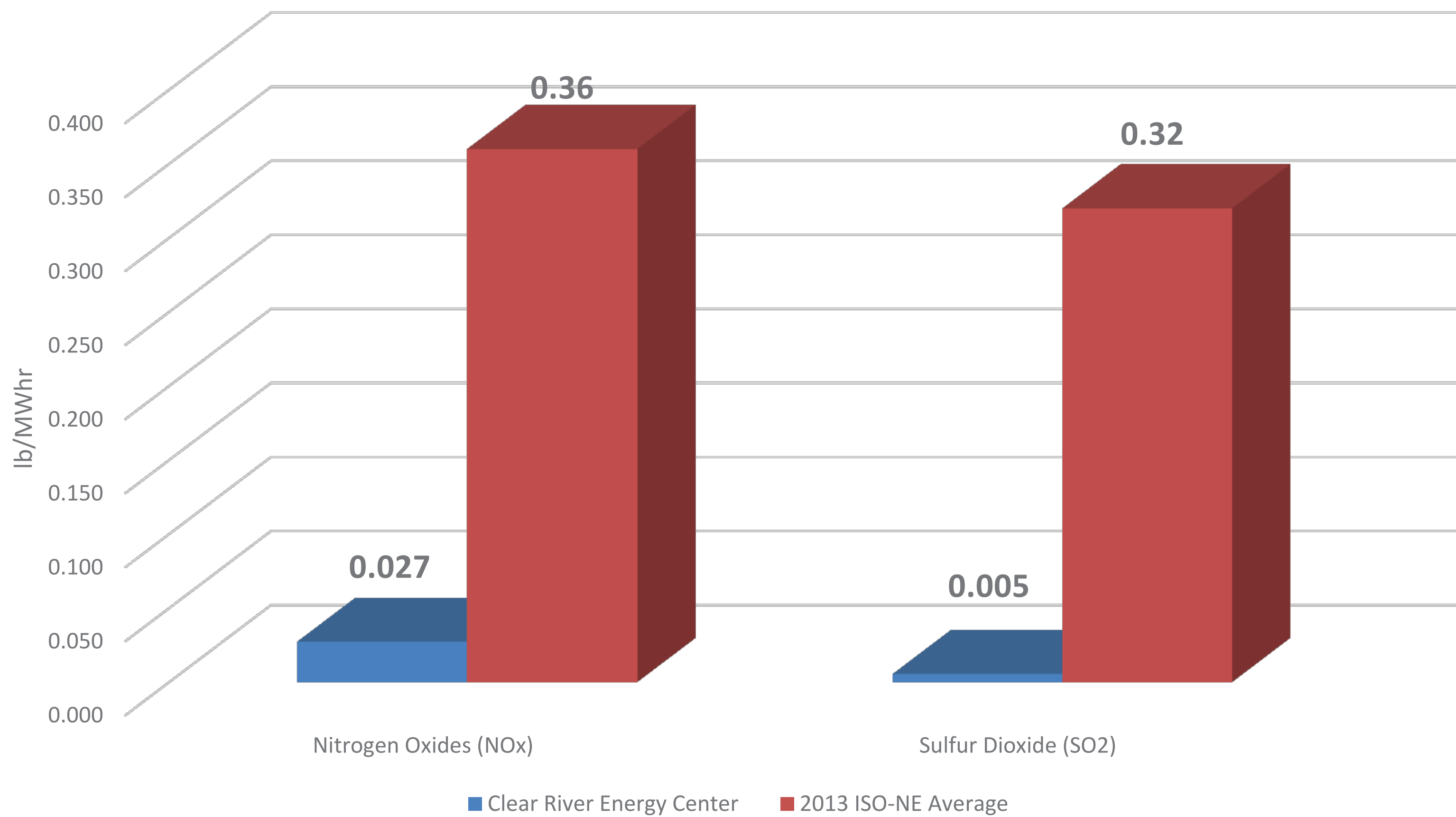
Clear River Energy Center Emissions vs. 2013 ISO-NE Average
